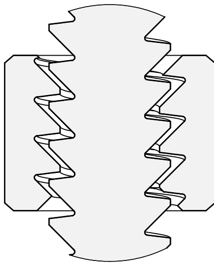
As assembled
